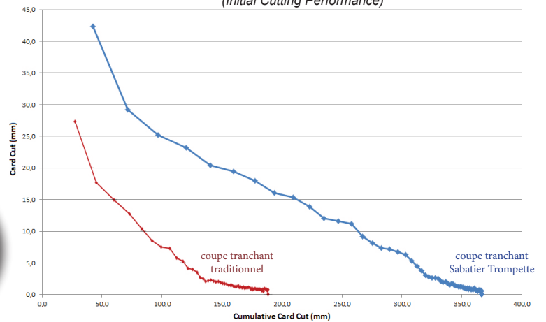
Comparatif tranchant - Norme ICP (Initial Cutting Performance)
